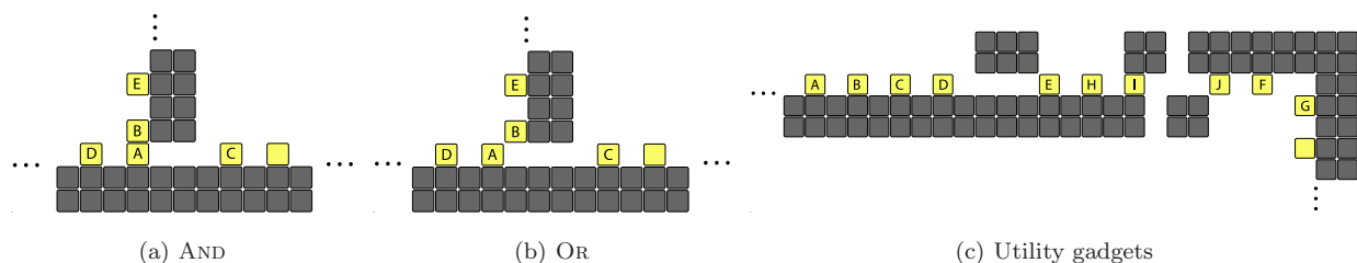
Figure 15: Sokoban gadgets.
