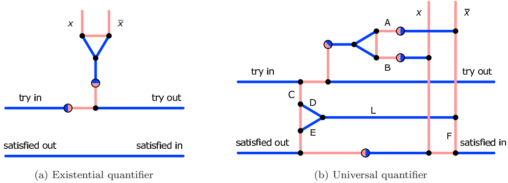
Figure 7: Quantifier gadgets.
