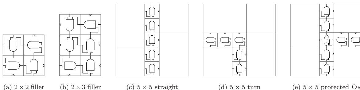
Figure 13: Sliding Blocks wiring.
